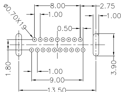
RECOMMENDED PCB LAYOUT TOP VIEW GENERAL TOLERANCE: T=1.60mm±0.05
